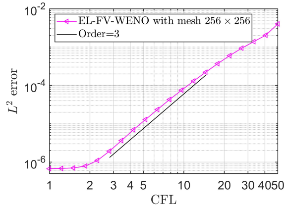
Figure 3.11: (Kelvin-Helmholtz instability problem) Log-log plot of CFL numbers versus L^2 errors with fixed mesh 256 \times 256 at t = 5 of the EL-RK-FV-WENO scheme.
