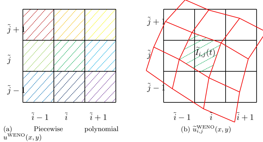
Figure 2.2: Schematic illustrations of u^{\text{WENO}}(x, y) and \tilde{u}_{i,j}^{\text{WENO}}(x, y) .
