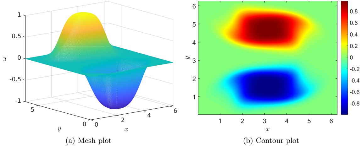
Figure 3.15: (Vortex patch problem) Mesh plot and contour plot of the numerical solution of the EL-RK-FV-WENO scheme with CFL = 10.2 and with mesh 256 \times 256 at t = 5 .
