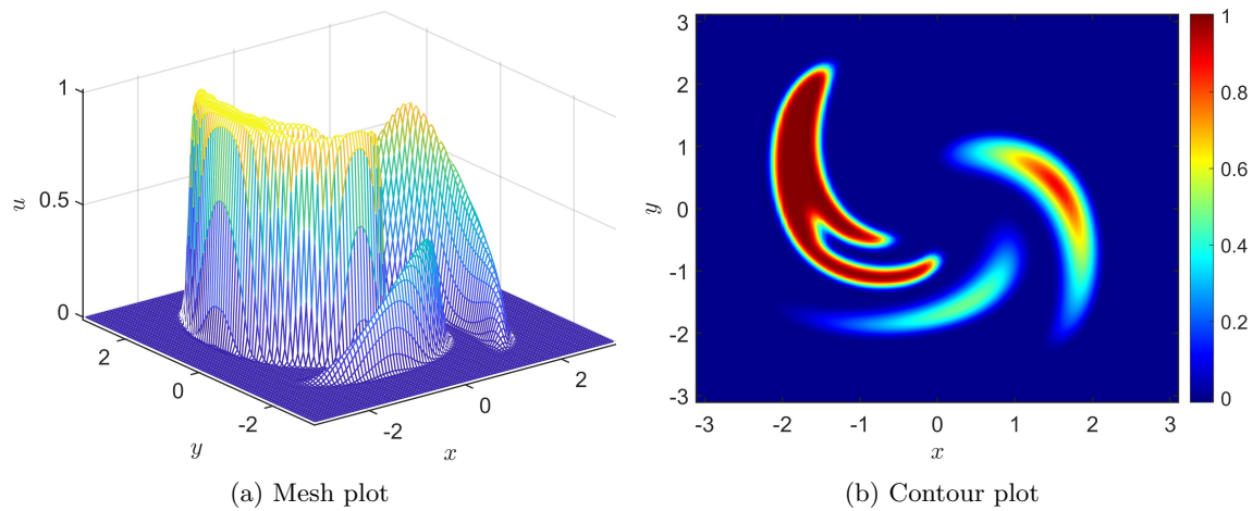
Figure 3.6: (Swirling deformation flow) Mesh plot and contour plot of the numerical solution of the EL-RK-FV-WENO scheme with CFL = 10.2 and mesh size 100 \times 100 at t = 0.75 .
