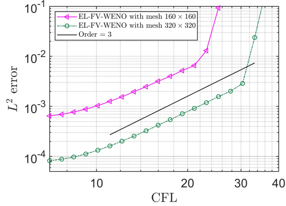
Figure 3.4: (Swirling deformation flow) Log-log plot of CFL numbers versus L^2 errors with fixed meshes 160 \times 160 and 320 \times 320 at t = 1.5 of the EL-RK-FV-WENO scheme.
