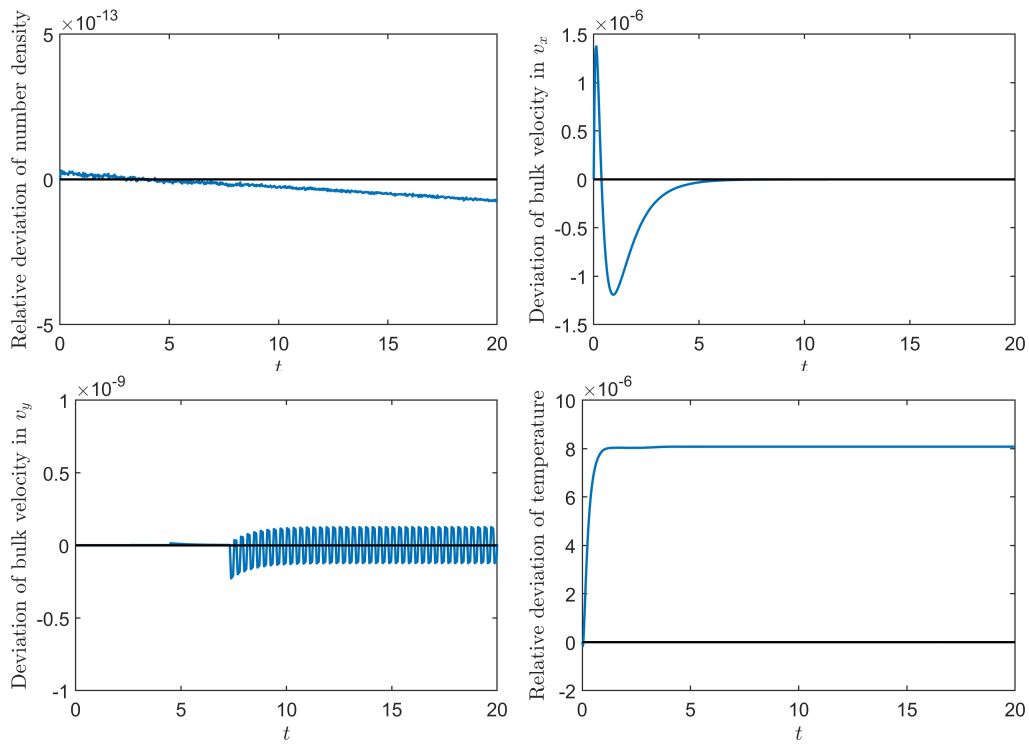
Figure 3.10: (The 0D2V Leonard-Bernstein linearized Fokker-Planck equation) Relative deviation (or deviation) of number density, bulk velocity in v_x , bulk velocity in v_y , and temperature for the EL-RK-FV-WENO scheme with CFL = 10.2 and with mesh 160 \times 160 from t = 0 to t = 20 .
