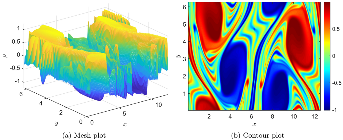
Figure 3.12: (Kelvin-Helmholtz instability problem) Mesh plot and contour plot of the numerical solution of the EL-RK-FV-WENO scheme with \text{CFL} = 10.2 and with mesh 256 \times 256 at t = 40 .
