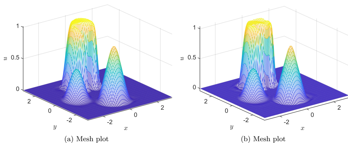
Figure 3.7: (Swirling deformation flow) Mesh plots of the numerical solution of the EL-RK-FV-WENO scheme (left) and WENO scheme in [38] using the same setting (right) with CFL = 10.2 and mesh size 100 \times 100 at t = 1.5 .
