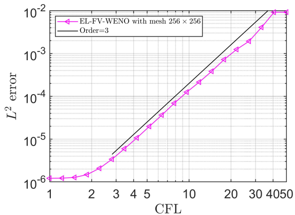
Figure 3.14: (Incompressible Navier-Stokes equations) Log-log plot of CFL numbers versus L^2 errors with fixed mesh 256 \times 256 at t = 0.5 of the EL-RK-FV-WENO scheme.
