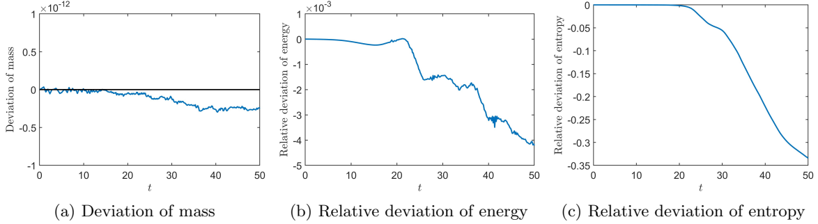
Figure 3.13: (Kelvin-Helmholtz instability problem) Deviation of mass, relative deviation of energy and entropy for the EL-RK-FV-WENO scheme with CFL = 10.2 and with mesh 256 \times 256 from t = 0 to t = 50 .
