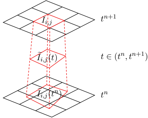
Figure 2.1: Schematic illustration for the dynamic region \tilde{I}_{i,j}(t) .
