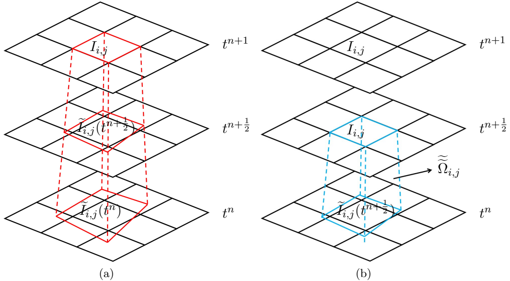
Figure 2.3: Schematic illustration of full discretization with IMEX(1,2,2).
