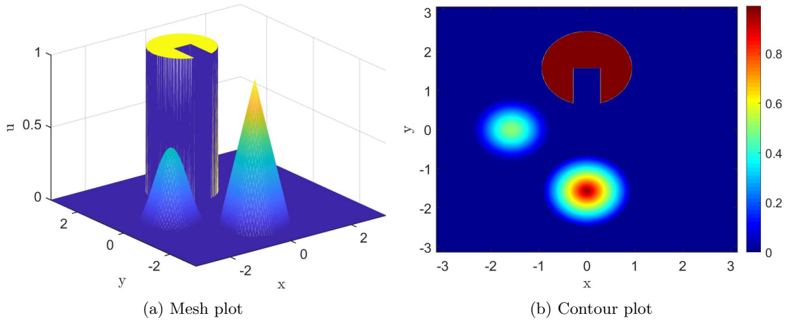
Figure 3.5: (Swirling deformation flow) Mesh plot and contour plot of a discontinuous initial condition.
